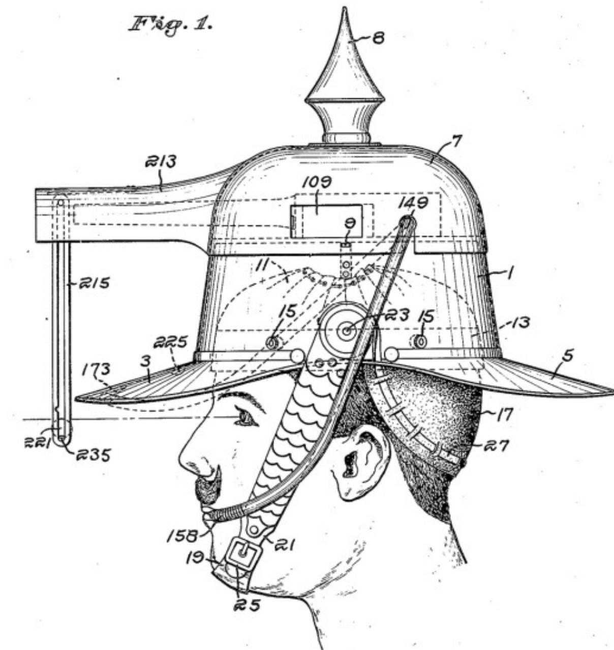
Head-mounted targeting and gun-firing interface: 1916
